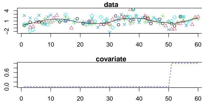
Fig. 19.12. Observations (points) of the true data (line) with covariate effect plus error and missing values added. It affects some time series positively and others negatively.
