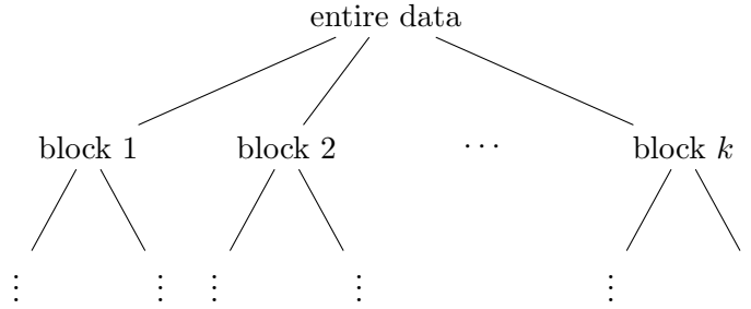
Figure 1: The user can define the second level of the tree structure using the argument block of the functions cluster_var / cluster_position and test_hierarchy if desired. In this example, there are k blocks on the second level of the tree. The function cluster_var / cluster_position builds a separate hierarchical tree for each of the blocks.
